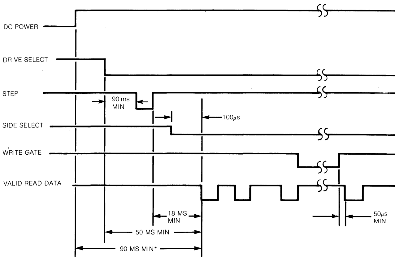
FIGURE 3. READ INITATE TIMING
