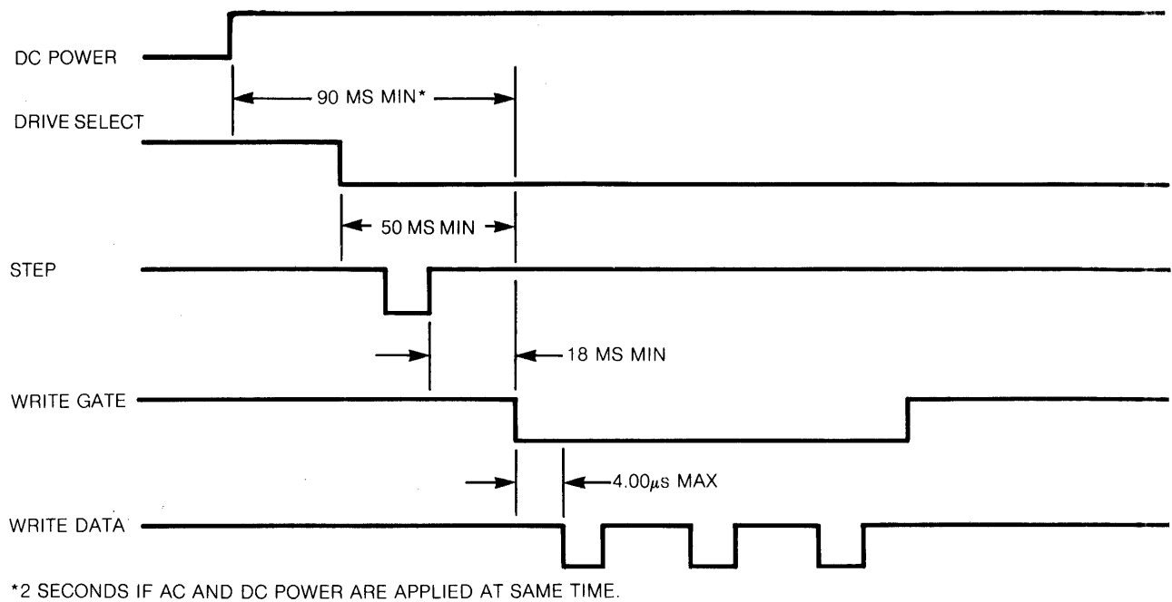
FIGURE 6. WRITE INITIATE TIMING
