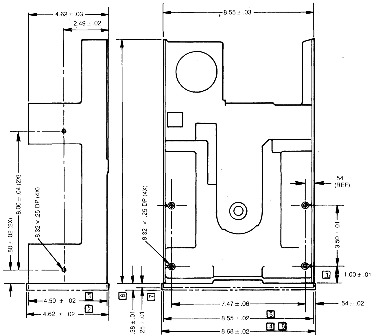
FIGURE 19. SA850/851R DIMENSIONS
