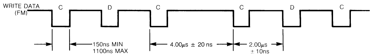
FIGURE 7. WRITE DATA TIMING (FM ENCODING)
