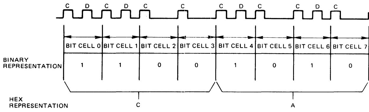
FIGURE 18. BIT CELL
