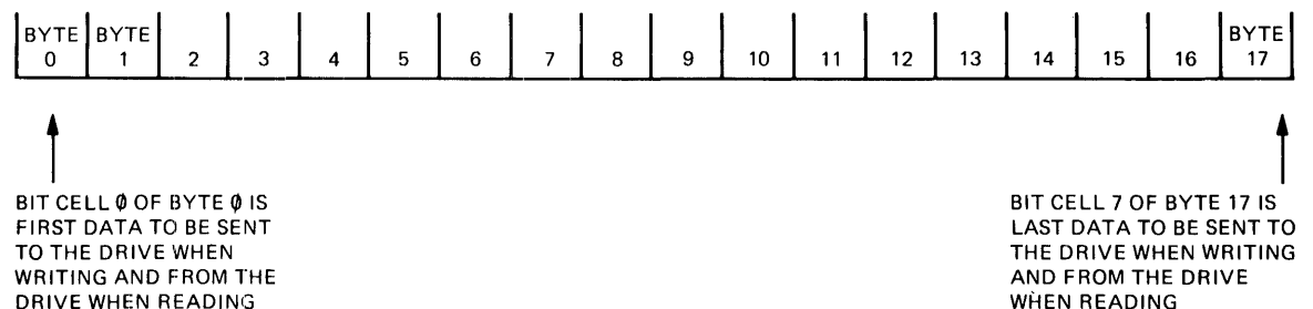
FIGURE 5. DATA BYTES
