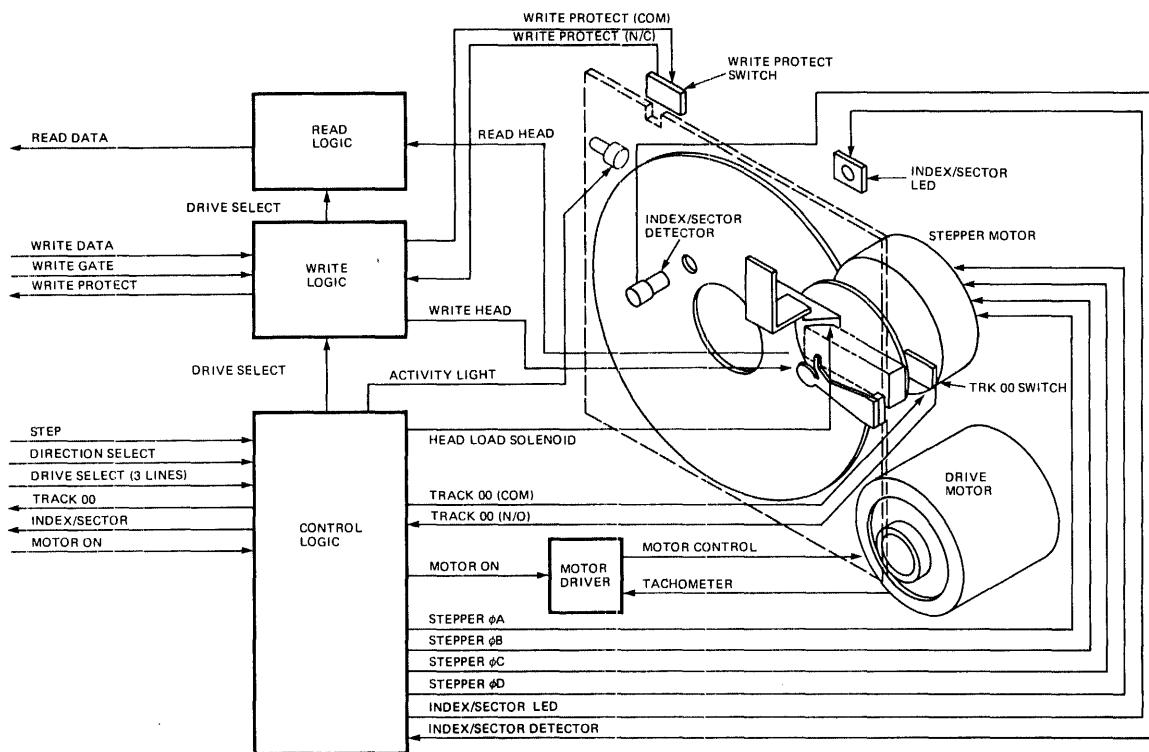
FIGURE 1. FUNCTIONAL DIAGRAM
