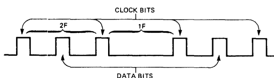
FIGURE 2. DATA PATTERN
