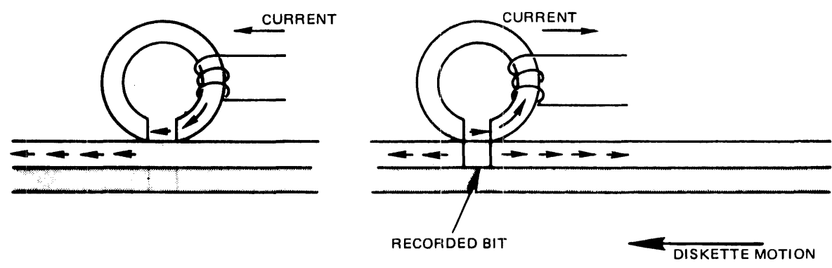
FIGURE 20. RECORDED BIT
