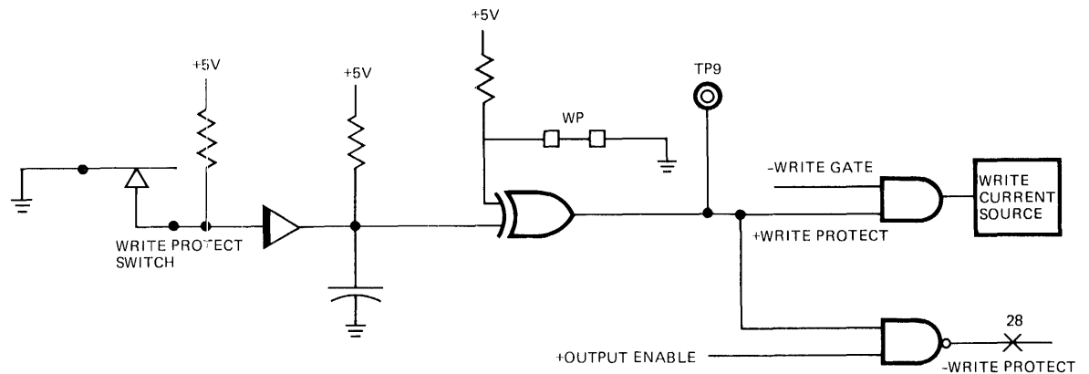
FIGURE 26. WRITE PROTECT FUNCTIONAL DIAGRAM
