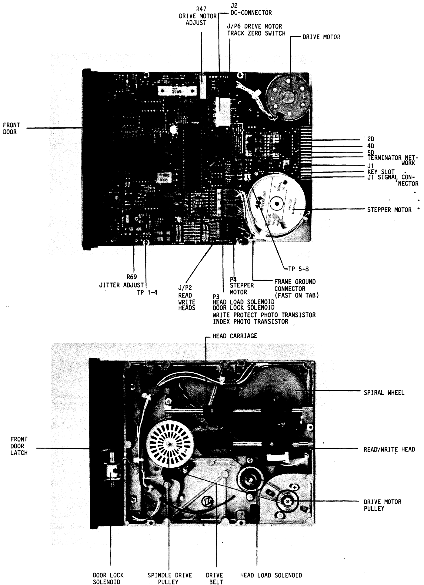
FIGURE 3 - 9 : PART LOCATIONS (PRINCIPAL)
