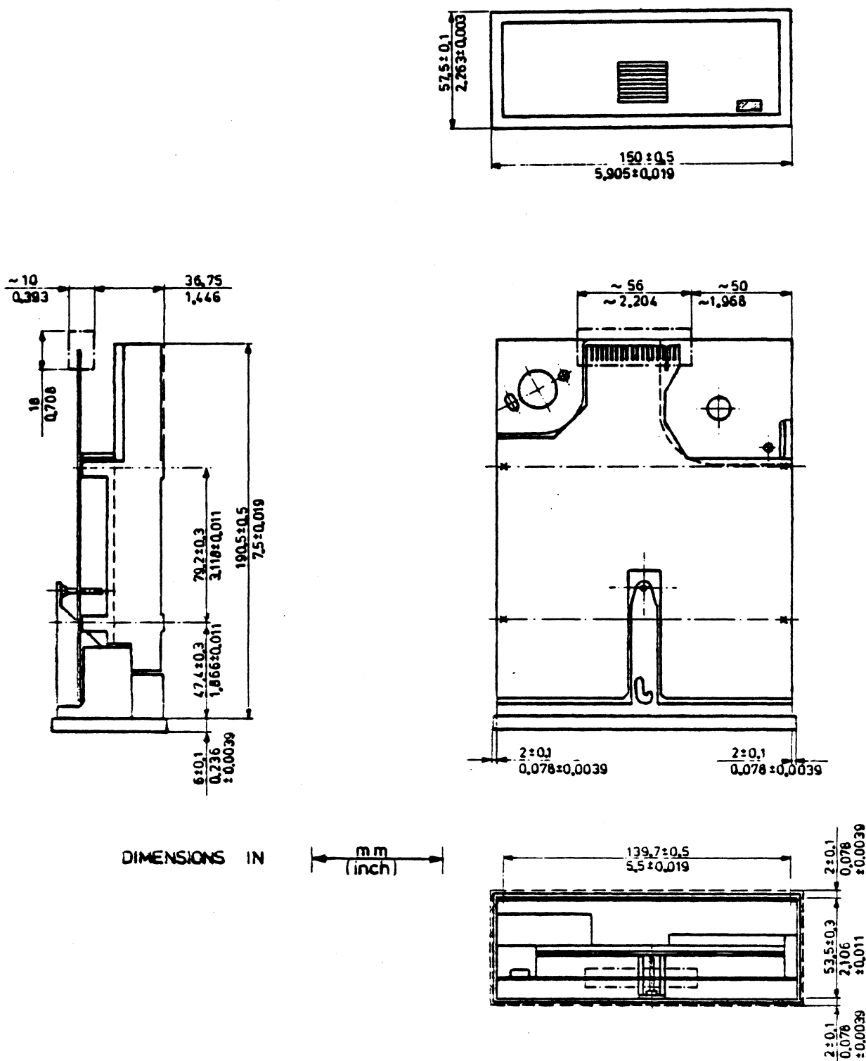
FIGURE 3 - 10 : MOUNTING SPECIFICATION
