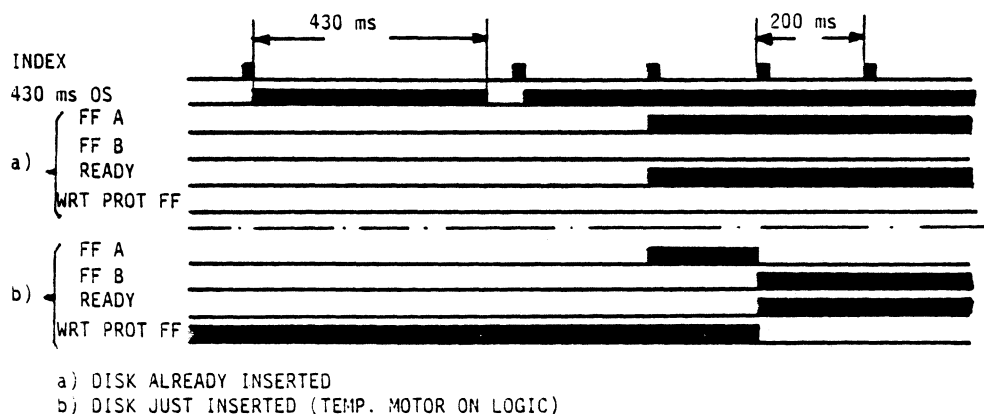
FIGURE 2 - 28 : READY TIMING
