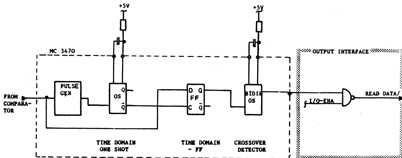
FIGURE 2 - 45 : TIME DOMAIN FILTER AND CROSSOVER DETECTOR
