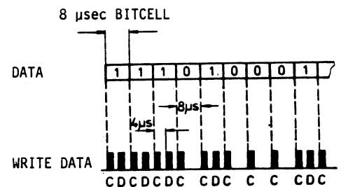
FIGURE 1 - 3 : FM-ENCODING
