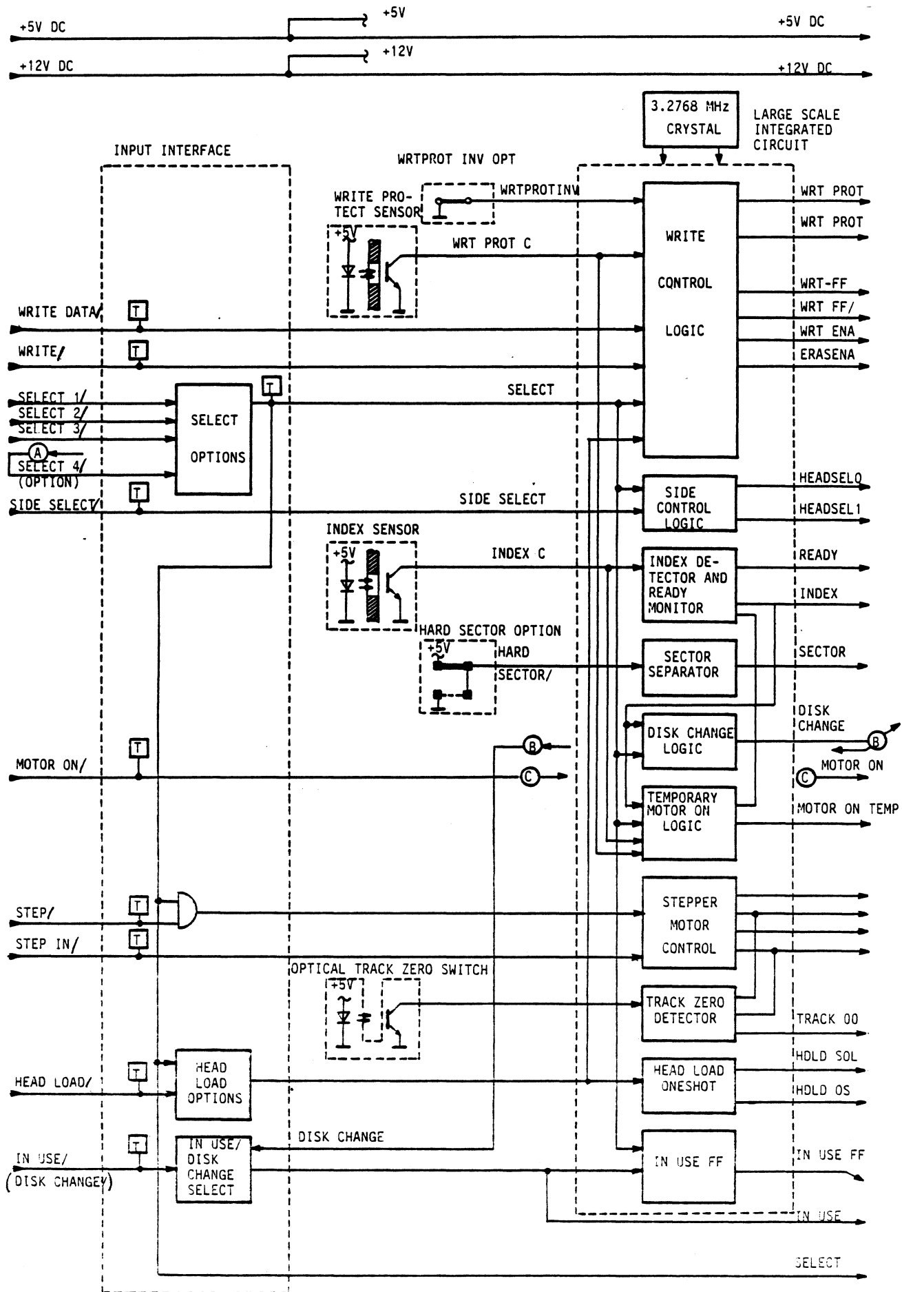
FIGURE 2 - 6 : BLOCK DIAGRAM
