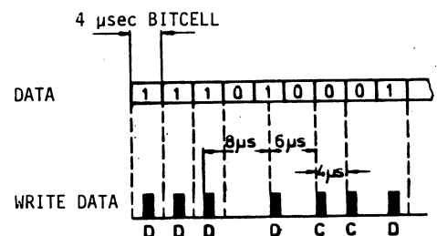
FIGURE 1 - 4 : MFM-ENCODING
