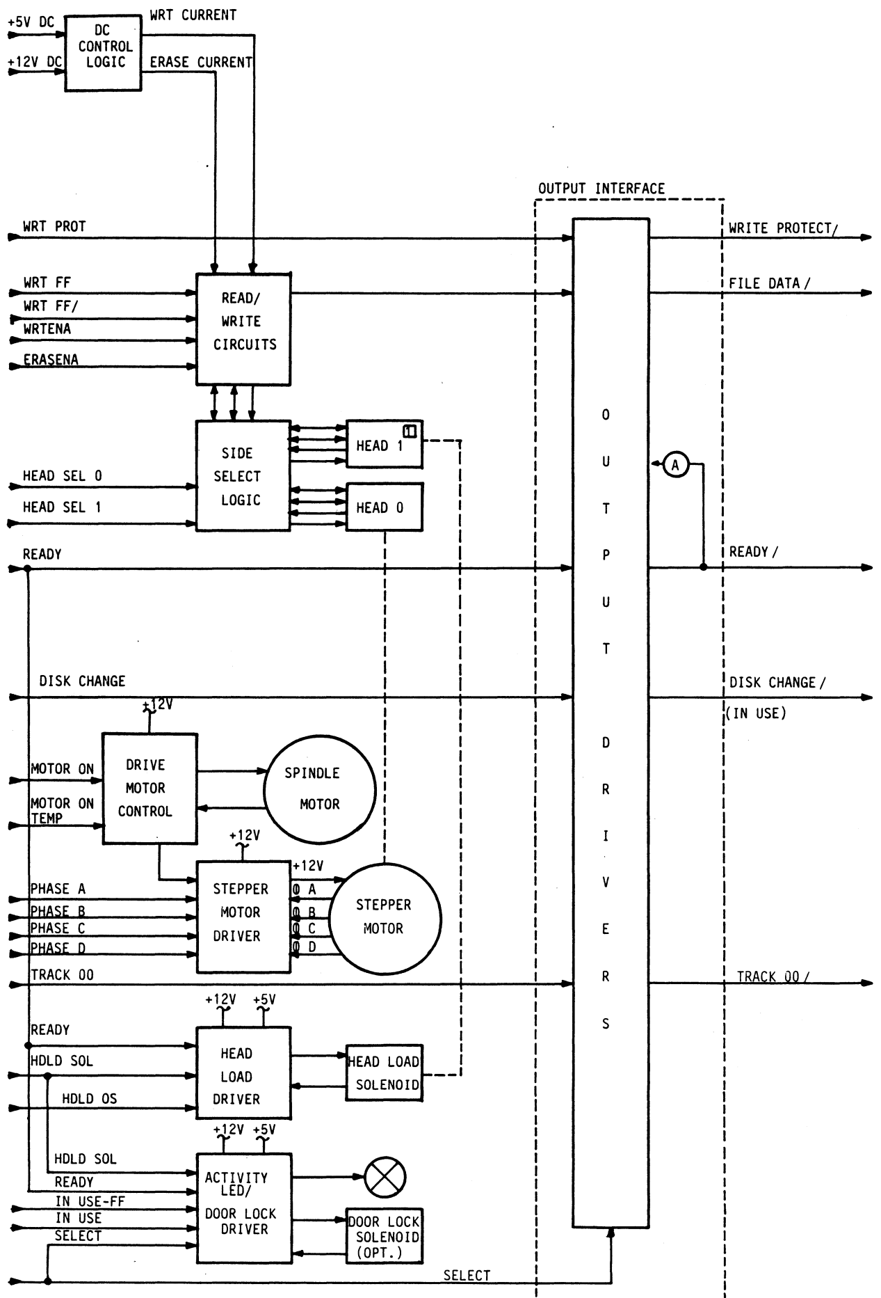
FIGURE 2 - 6 : BLOCK DIAGRAM
