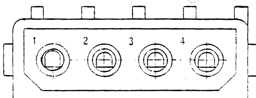
FIGURE 3 - 2 : DC-CONNECTOR
