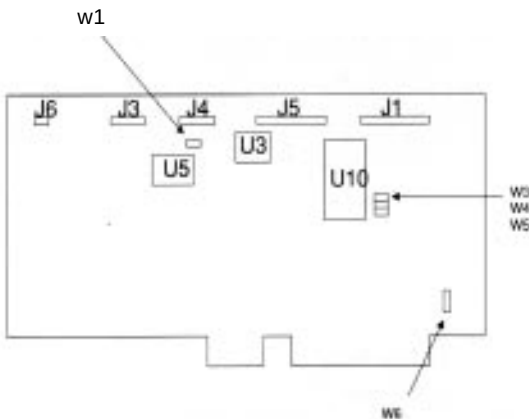
All jumpers OFF for factory defaults.
